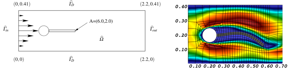
Figure 59: Left: Flow around a cylinder with an elastic beam described by a nonlinear wave equation [75]. Right: Snapshot of the numerical solution of the velocity field. Both figures copied from [133].
