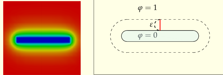
Figure : Sneddon's 3D stationary pressurized fracture: Fracture representation using the phase field \varphi . The inner blue region indicates the crack with \varphi = 0 and the red region indicates the unbroken zone where \varphi = 1 . We have a diffusive zone in between (green region).
