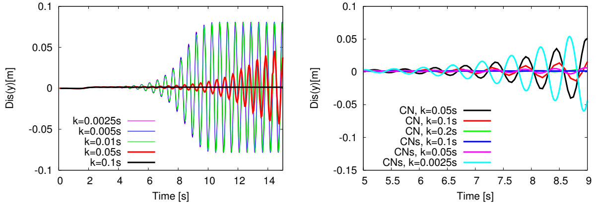
Figure 60: Taken from [133]: Comparison of u_y (tip of the elastic beam in y direction) on mesh level 1 and different time step sizes k using the shifted Crank-Nicolson (CNs) scheme (left) and a comparison with the classical Crank-Nicolson (CN) method (right). First thanks to the monolithic formulation and implicit time-stepping we are able to use large time steps, e.g., k = 0.2s . Secondly, the large time step is not sufficient any more to lead to the correct oscillations of the elastic beam. In particular, care of the correct choice of the damping factor using the shifted version must be taken. From this figure, we infer that the largest time step size is around k \sim 0.01s in order to obtain the correct amplitude of oscillations.
