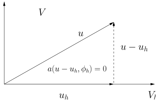
Figure 24: Illustration of the Galerkin orthogonality.
