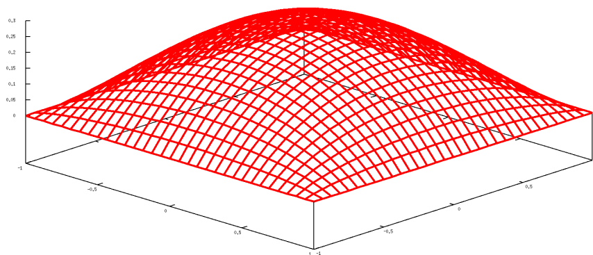
Figure 2: Solution of the Poisson problem on \Omega = (-1, 1)^2 with the right hand side f = 1 .
