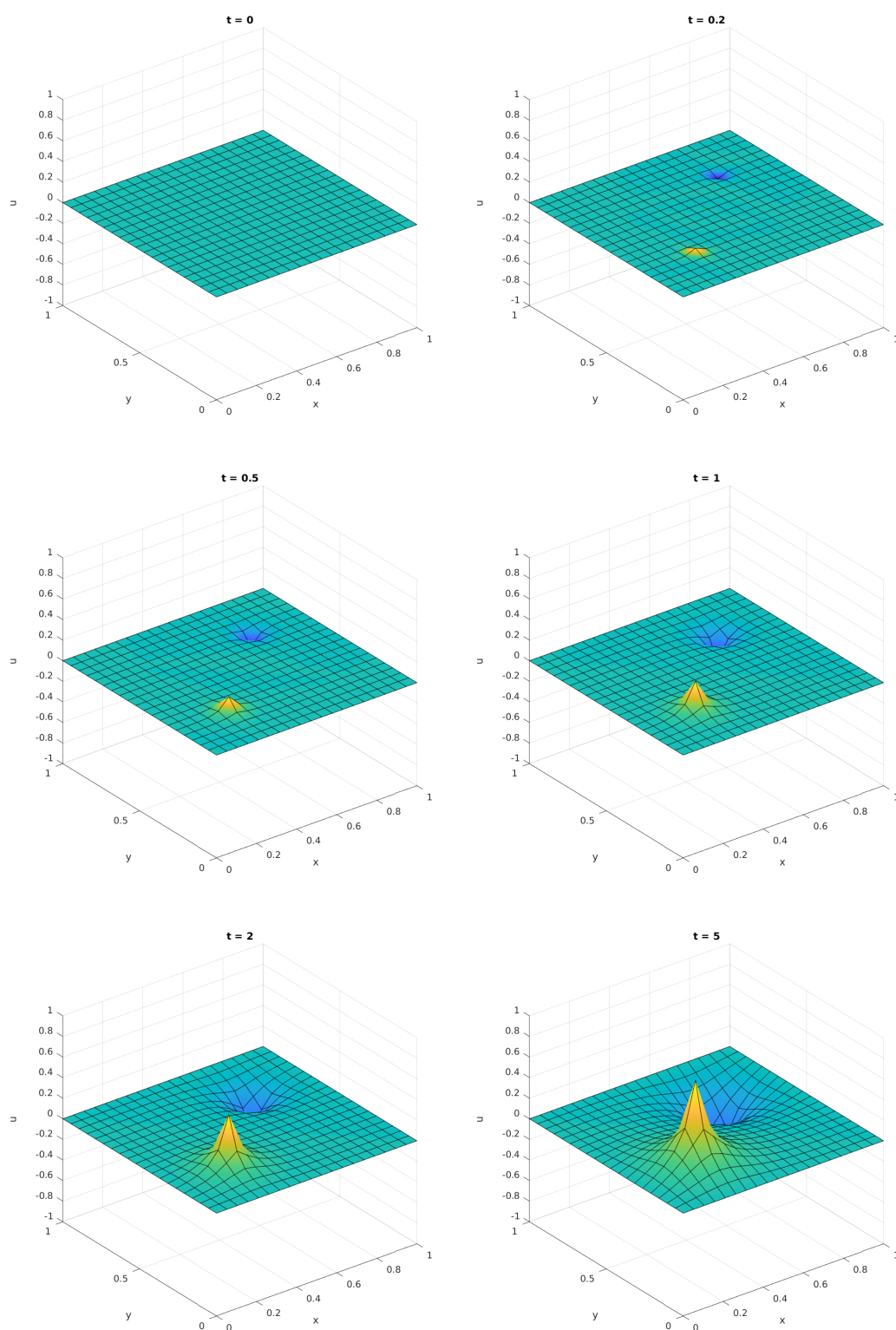
Figure 53: Numerical simulations using the shifted Crank-Nicolson scheme. Solution plots at t = 0, 0.2, 0.5, 1, 2, 5 are displayed. Here, we observe stable results. Figures provided by [58].
